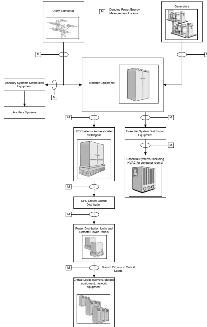
Fig. 3 Minimum Power/Energy Measurements for Assessing Energy Efficiency for a Typical Data Center
