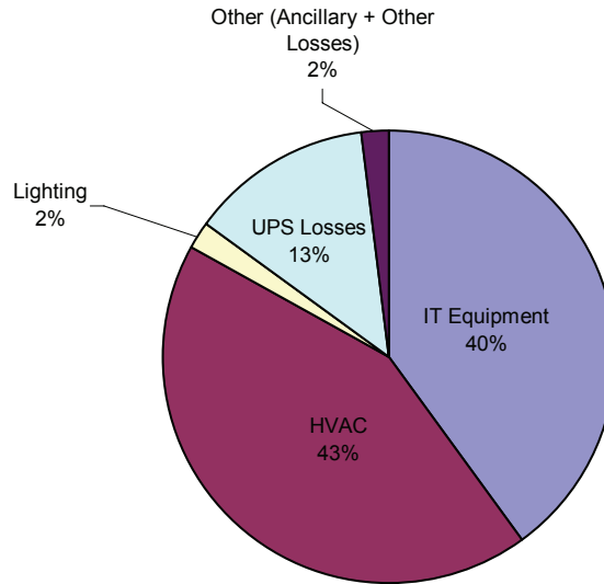
Fig. 2 Representative Data Center Gross Electrical Load Makeup
